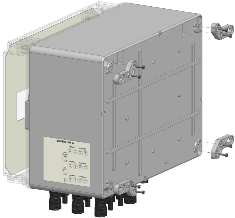
WALL FIXING HOLES FOR HORIZONTAL BRACKETS
