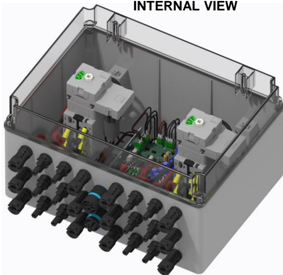
INTERNAL VIEW
